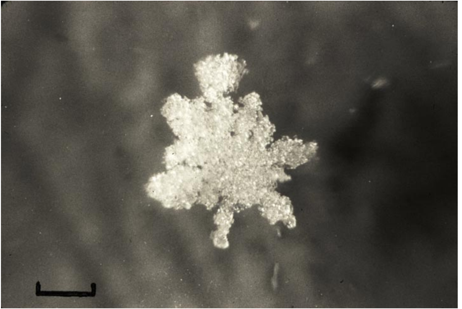
GRAUPEL PARTICLE IN NATURAL CLOUDS OVER THE CASCADE MOUNTAINS
