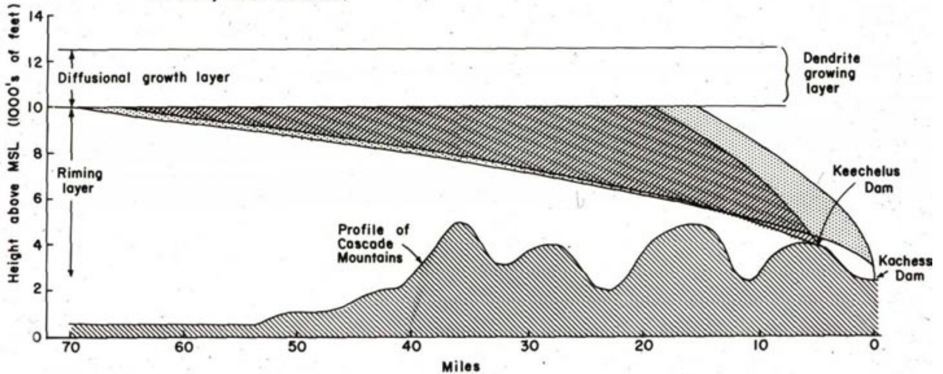
Cross section of trajectories for dendrites falling at Keechelus Dam and Kachess Dam at 1515 PST on February 3, 1971. (▨ Densely rimed dendrites ▩ Moderate to densely rimed dendrites)
