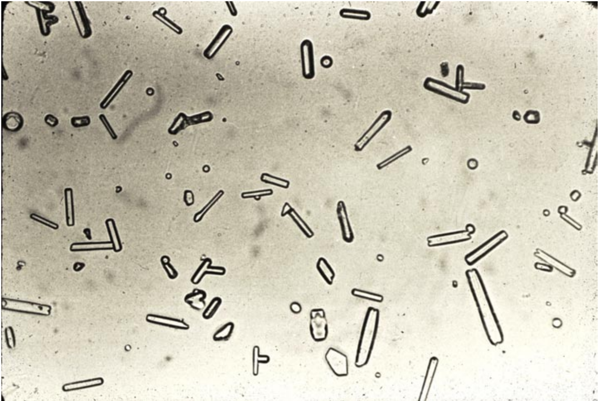
UNRIMED COLUMN CRYSTALS PRODUCED BY HEAVY ARTIFICIAL SEEDING OVER THE CASCADE MOUNTAINS
