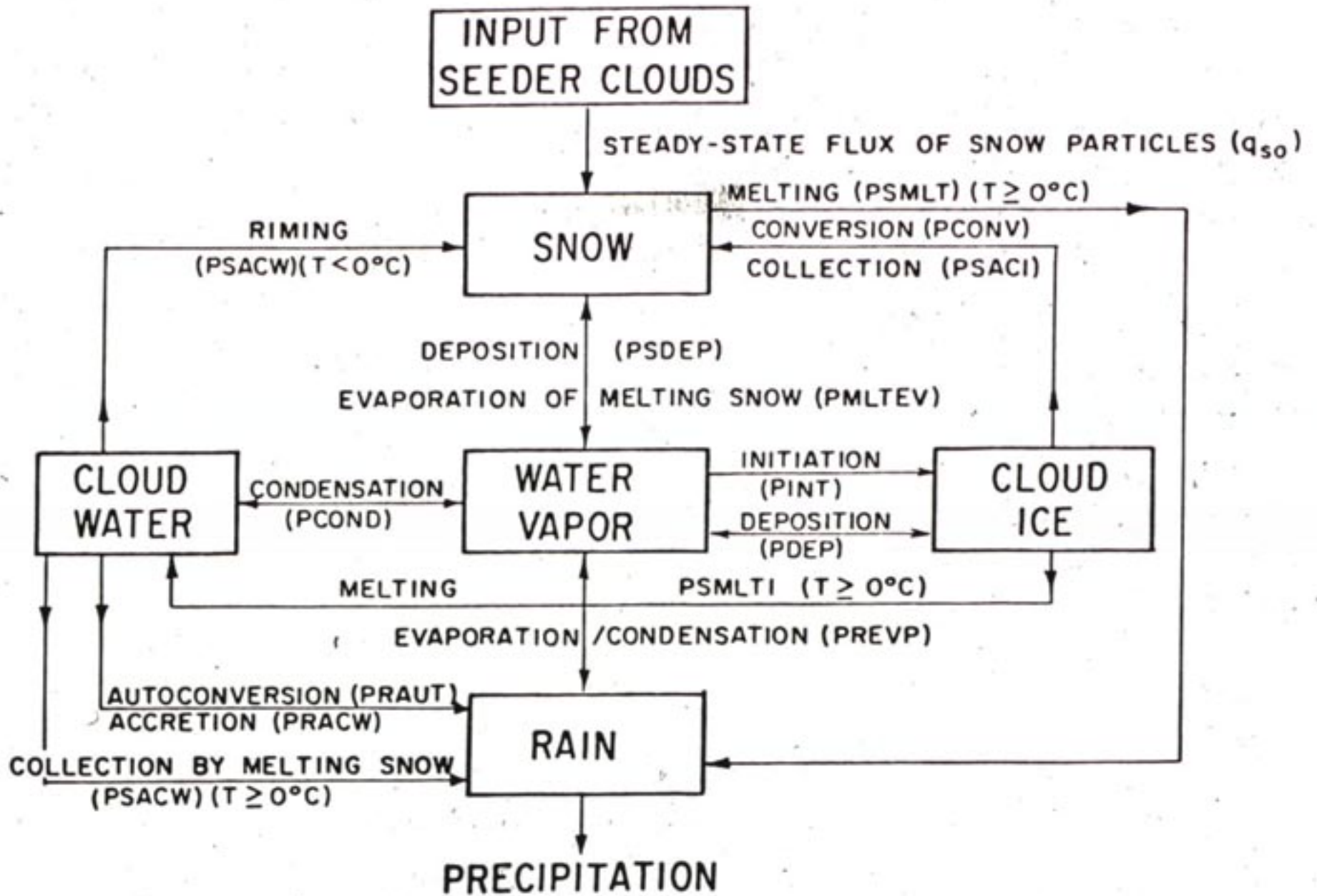
Rutledge & Hobbs Cloud Parameterization Scheme
