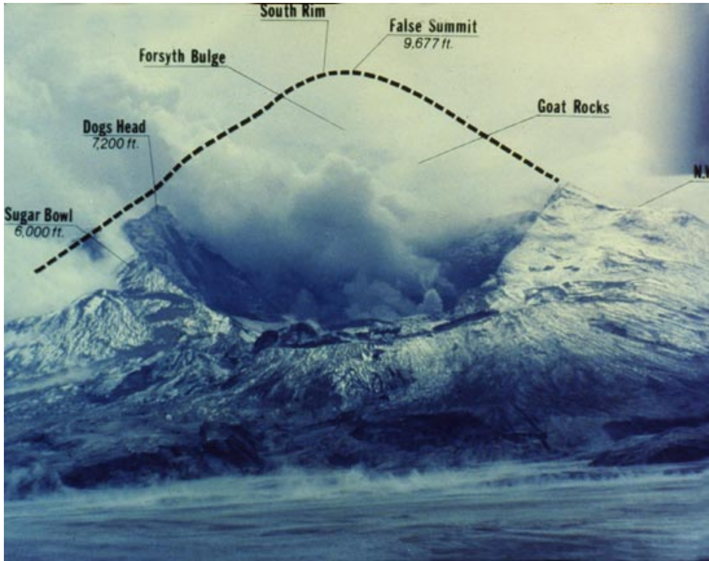
Mt. St. Helens 18 May 1980
