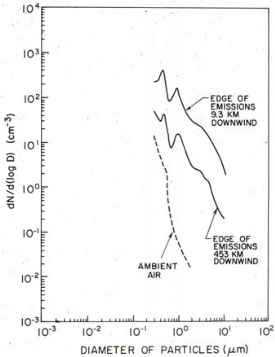
PARTICLE SIZE SPECTRA MEASURED IN ASH EMISSIONS FROM MT. ST. HELENS ON MAY 18, 1980
