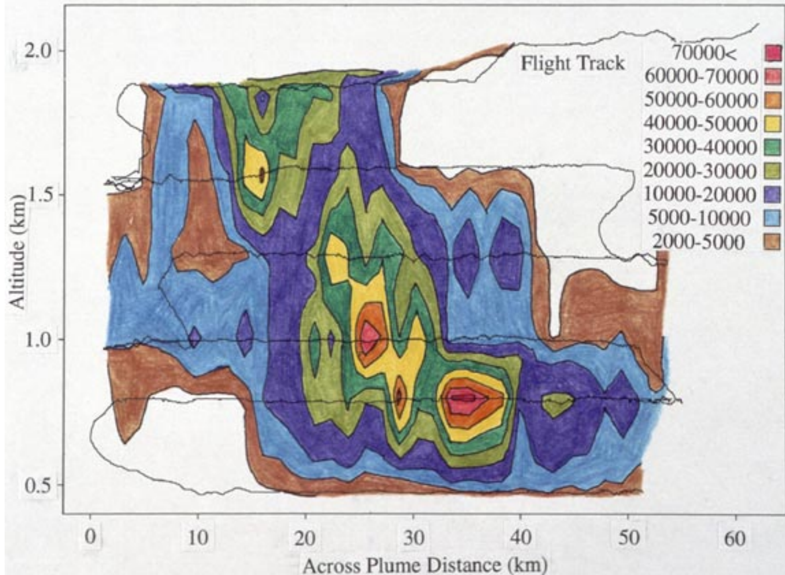
CROSS-SECTION OF COMPOSITE KUWAIT SMOKE PLUME 40 KM DOWNWIND OF FIRES Showing Total Particle Concentrations ( \text{cm}^{-3} )
